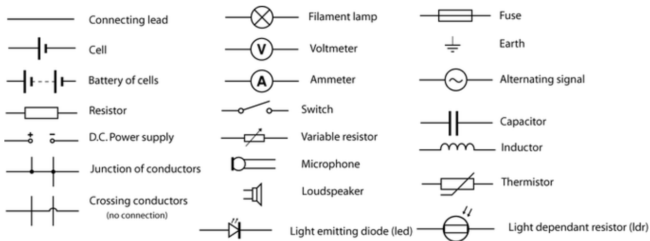
A set of example circuit elements and their associated symbols in common use Source: Wikibooks licensed under: CC BY-SA 3.0
