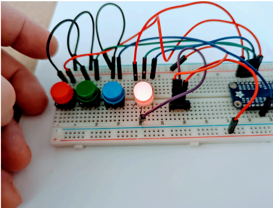
Digitally switched RGB LED with red, green, and blue legs of the RGB connected directly to their assigned GPIO ports.
