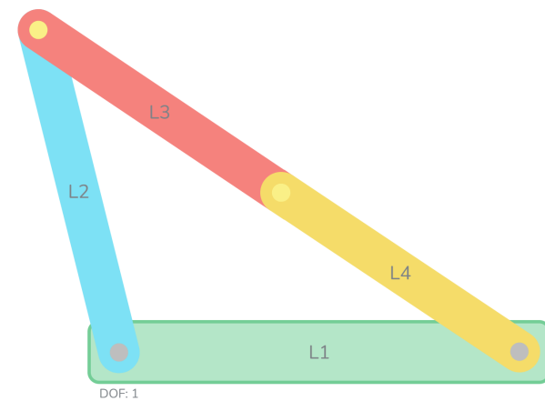
Toggle position for a non-Grashof mechanism
