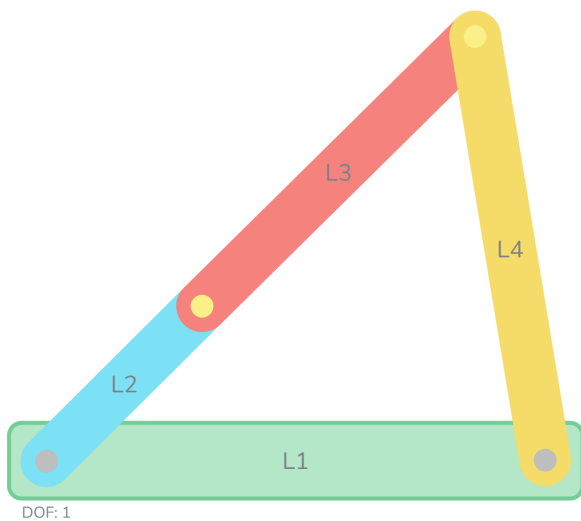
Toggle position for a non-Grashof mechanism
